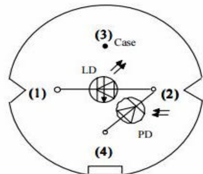
Pin Connection ( Top view )
